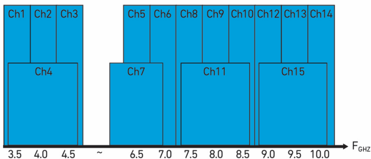
Figure 11: UWB frequencies.
